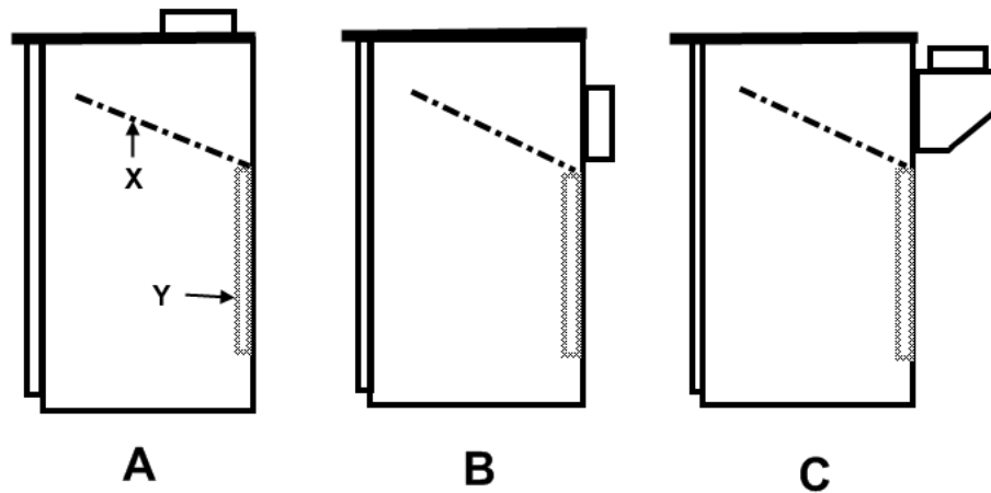
Diagrams showing the flue outlet from the top (A), back (B) and back box (C). X = Position of baffle plate Y = Back protection brick
